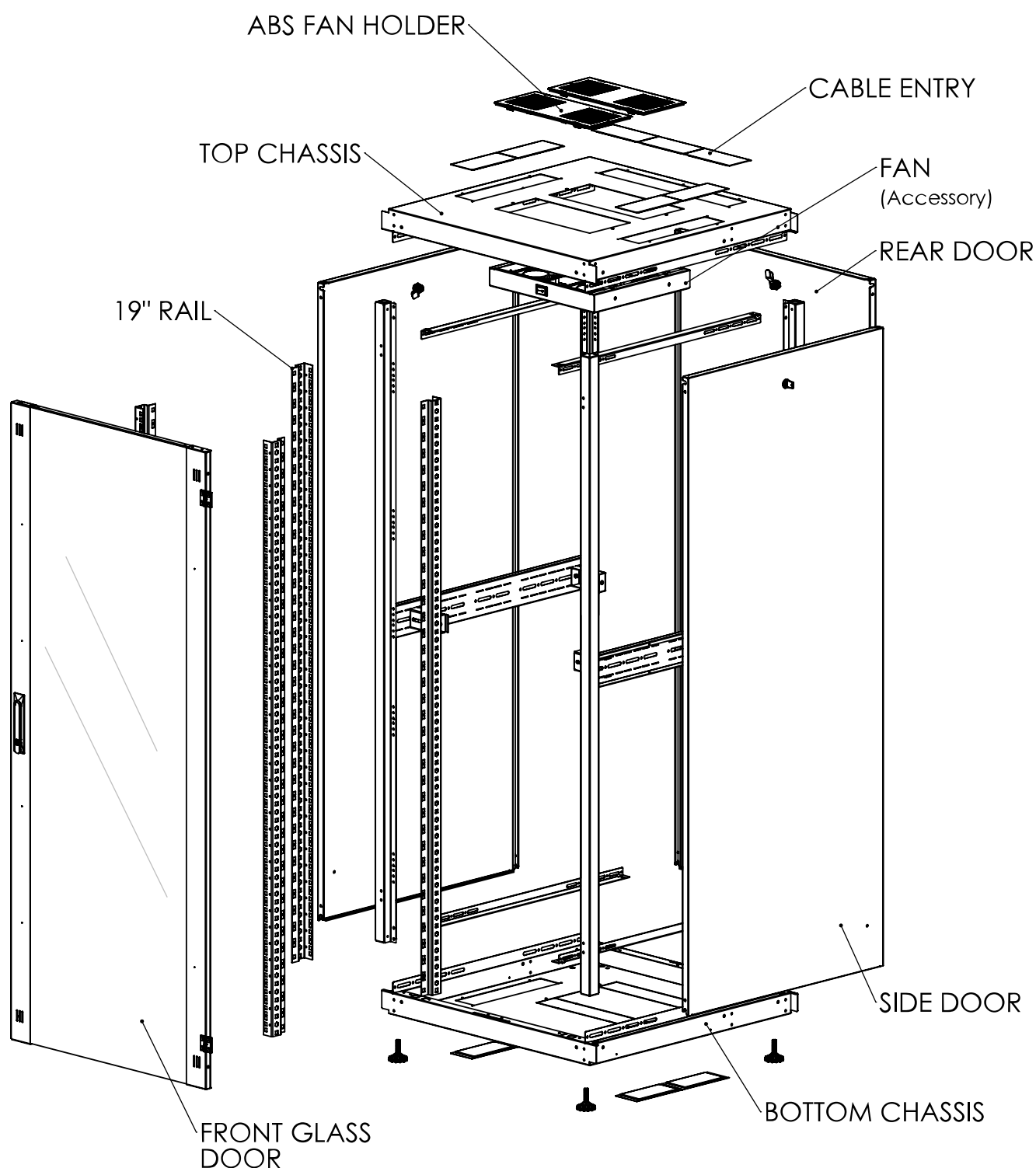
Exploded view
